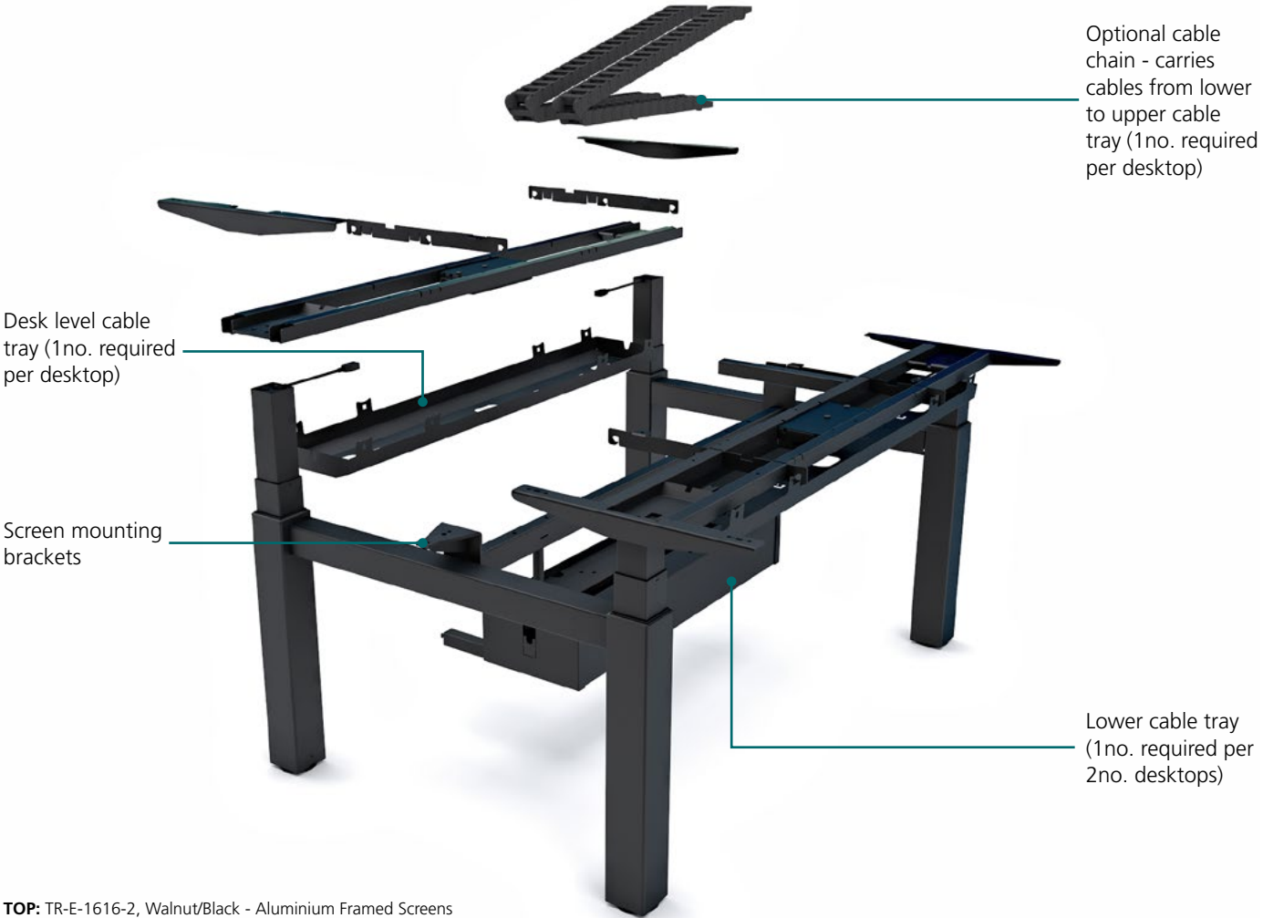
TOP: TR-E-1616-2, Walnut/Black - Aluminium Framed Screens BOTTOM: TR-E-1616-2, Black - exploded diagram
