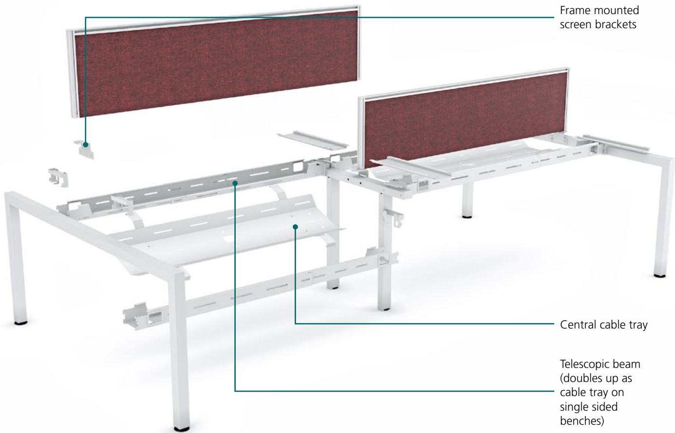
LNS-3216-4, White framework - exploded diagram
